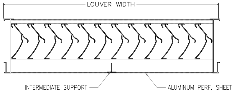
SECTION A
