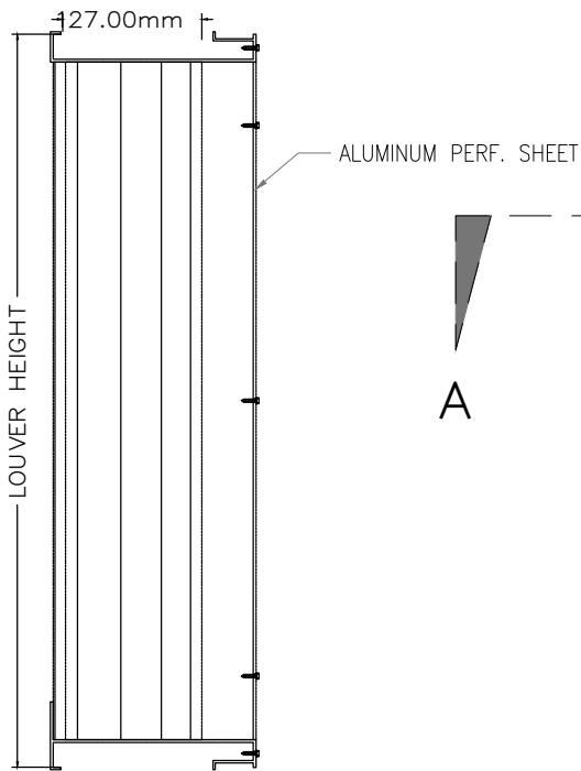
SECTION B
