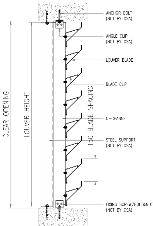
SECTION B
