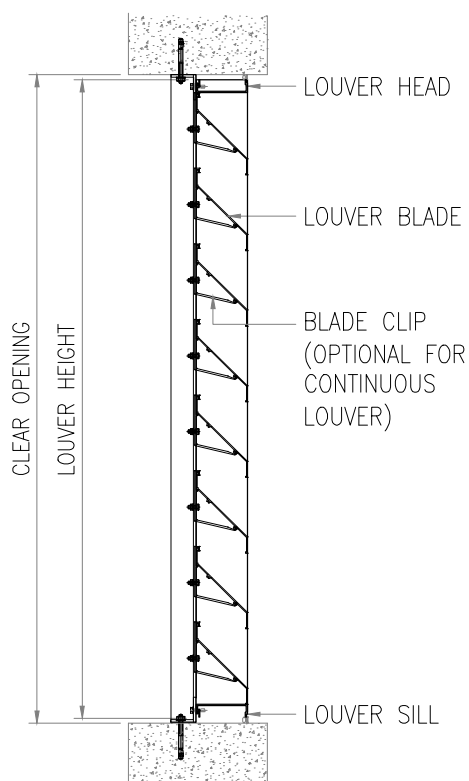
SECTION B
