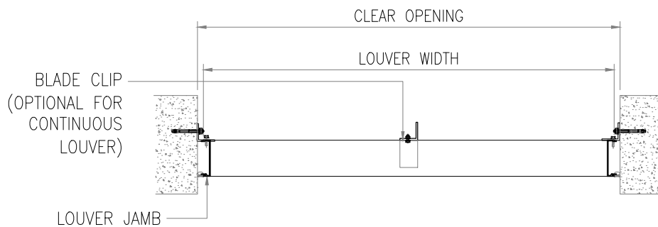
SECTION A
