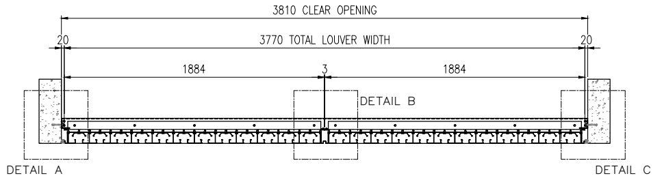
SECTION A
