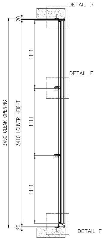
SECTION B
