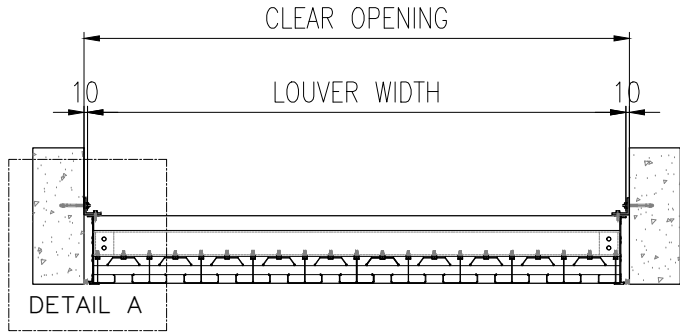
SECTION B
