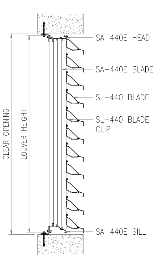
SECTION B
