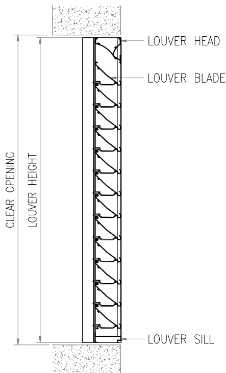
SECTION B
