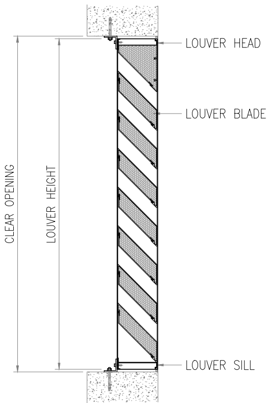
SECTION B
