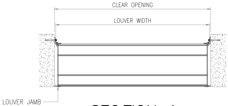
SECTION A
