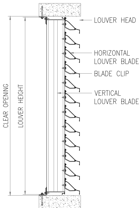
SECTION B
