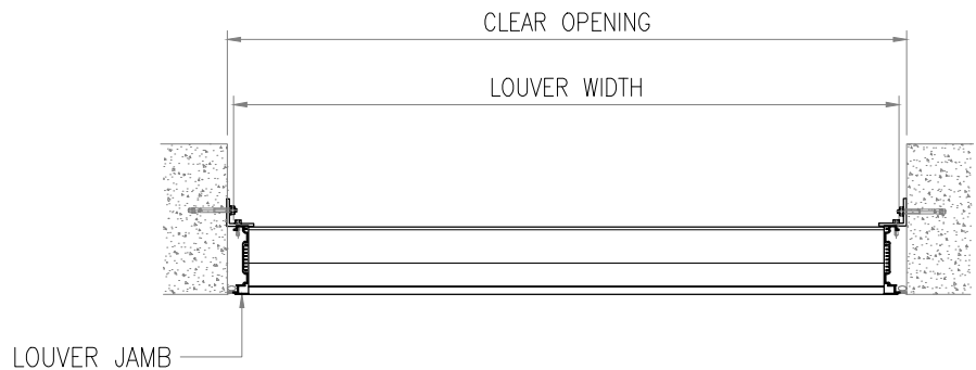
SECTION A
