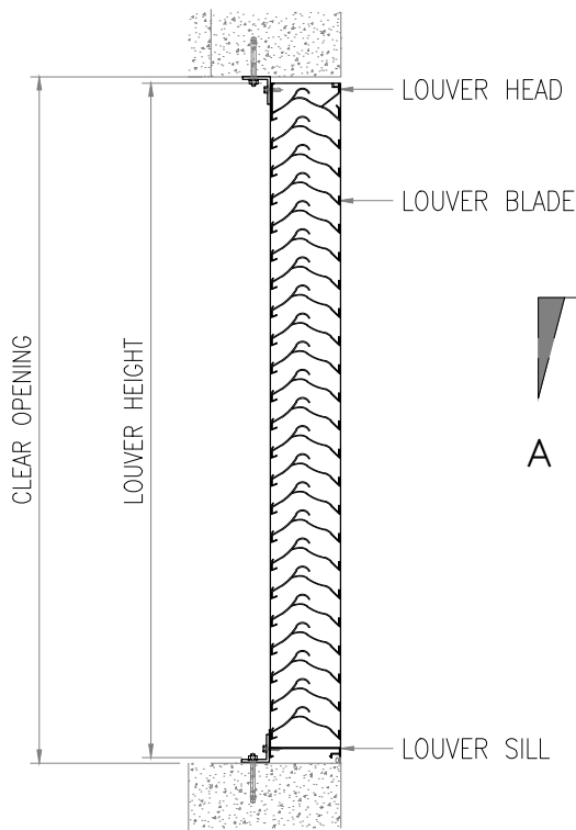
SECTION B
