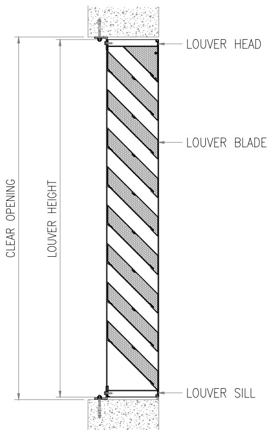
SECTION B
