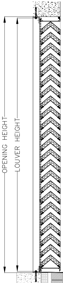
SECTION
