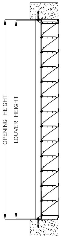
SECTION
