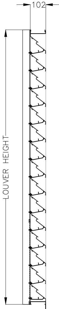
SECTION
