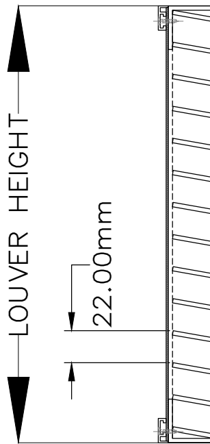
SECTION
