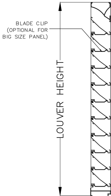
SECTION
